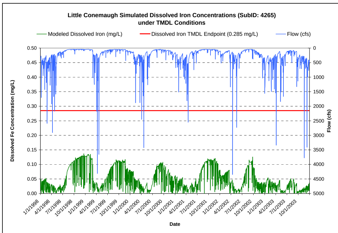
Figure 6-4. Simulated Dissolved Iron Concentrations under TMDL Conditions in the Little Conemaugh River Watershed.
