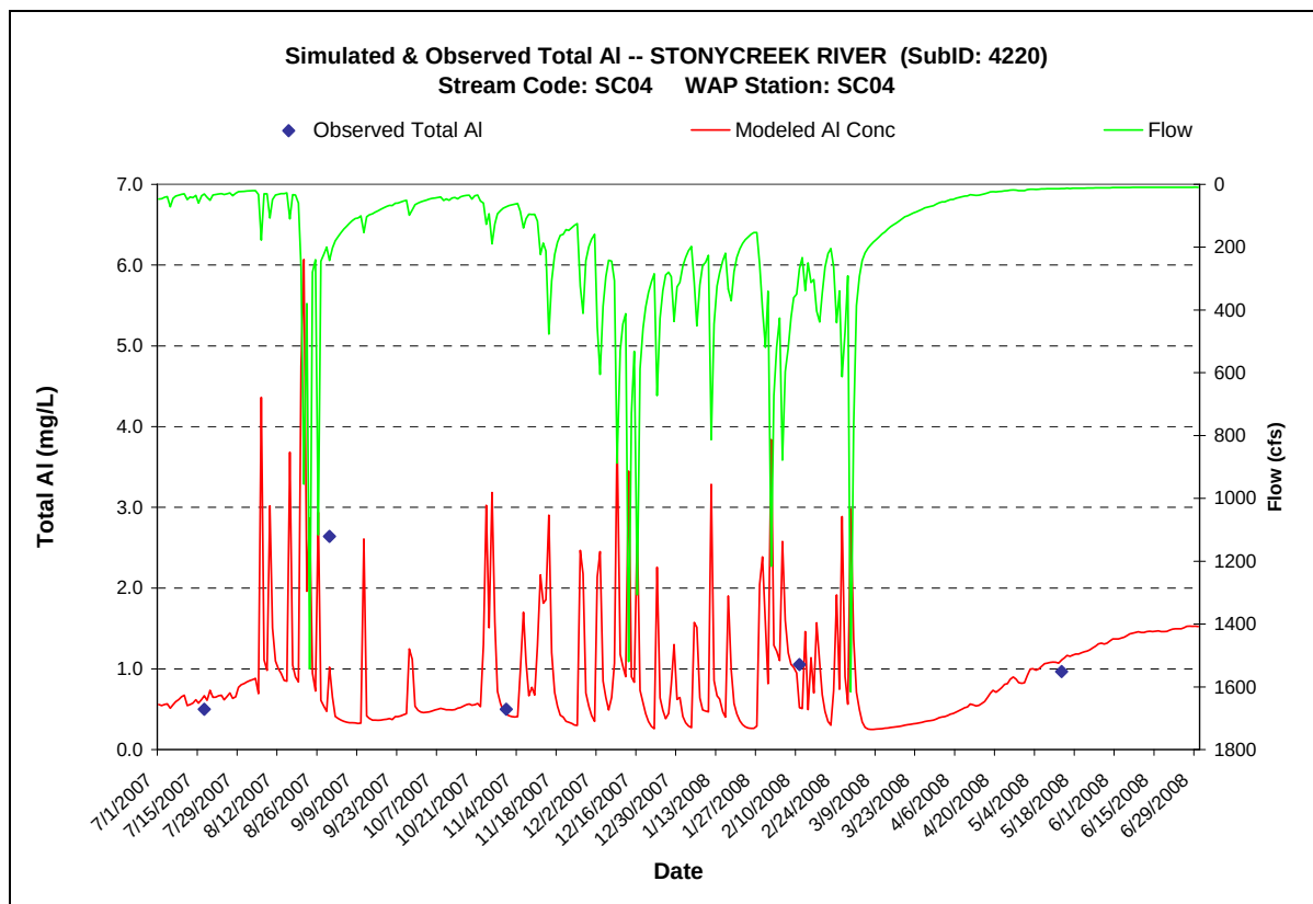
Figure 5-12. MDAS Water Quality Calibration for Aluminum at SC04, 2007–2008.
